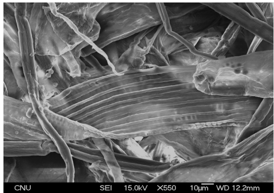
Fig. 1. Surface of handsheet paper made of the corn bast fibers detected by SEM (X 100, X 550).
