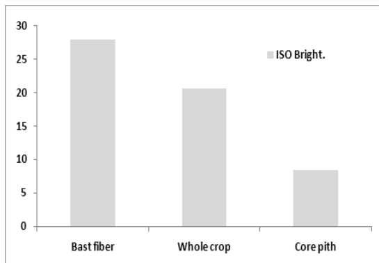
Fig 4. The Optical properties of handsheet paper made of corn stalk pulp.
