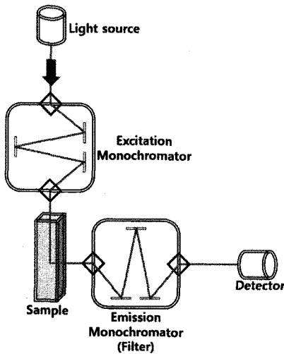
Fig. 3 Diagram of spectrofluorometer.
