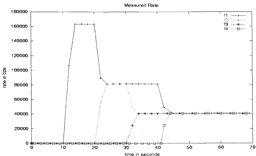
Figure 10. Simple Flows Evaluation for Non-Handover.
