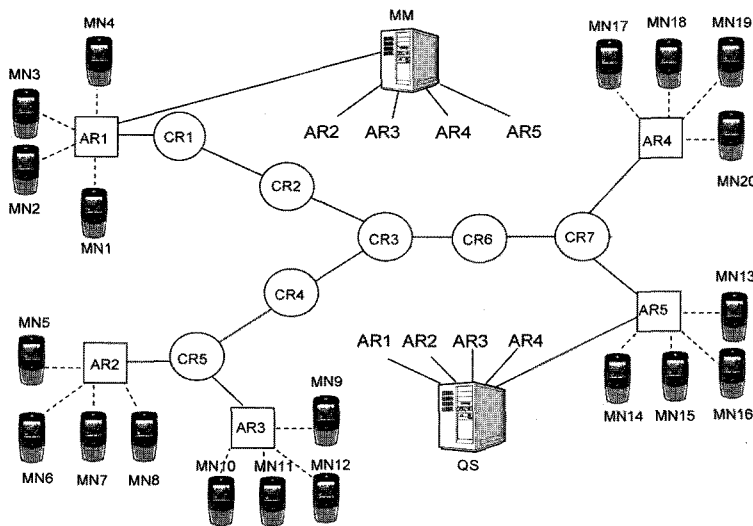
Figure 9. Simulated Network Topology.
