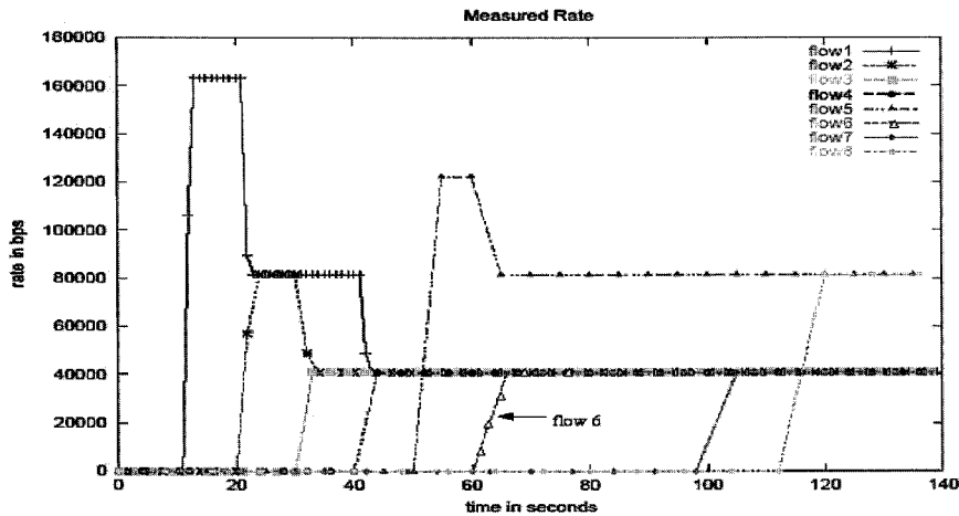
Figure 12. Multiple Flows Evaluation for Handover.
