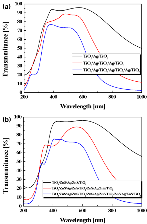
Fig. 2. The optical design by using EMP simulation with different stacking layers: (a) TiO 2 /Ag/TiO 2 structure, and (b) TiO 2 /ZnS/Ag/ZnS/TiO 2 structure.
