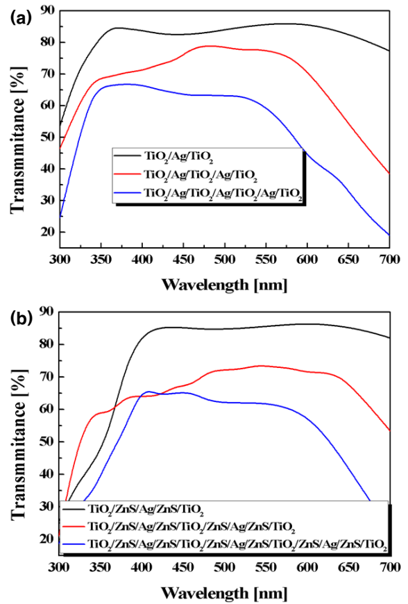
Fig. 3. Transmittance results of multi-layered films measured in the visible range: (a) TiO 2 /Ag/TiO 2 structure, and (b) TiO 2 /ZnS/Ag/ZnS/TiO 2 structure.
