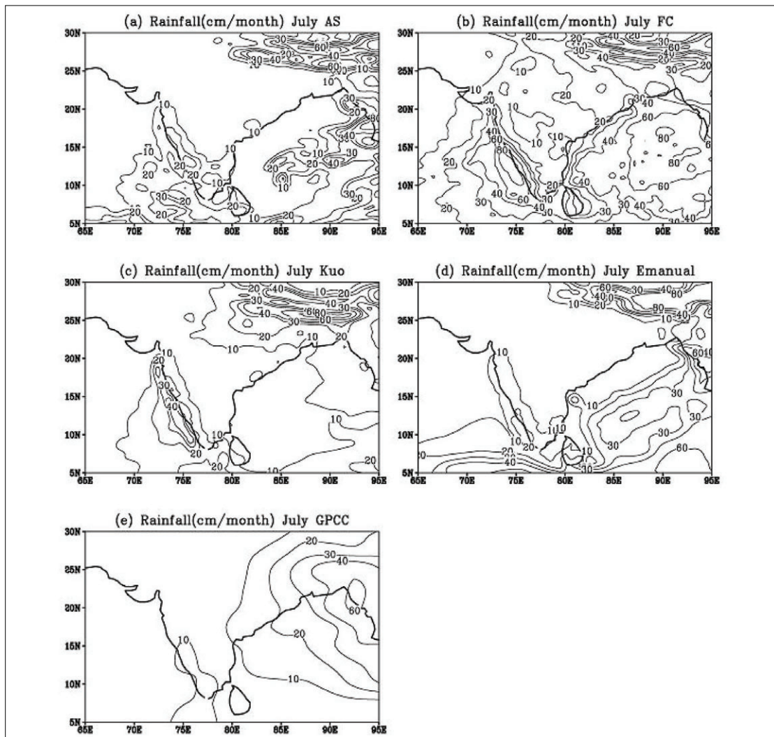
Fig. 2. Precipitation (cm) in July for (a) AS closure in Grell, (b) FC closure in Grell, (c) Kuo-type, (d) Emanuel schemes in RegCM3 and (e) observed from GPCC
