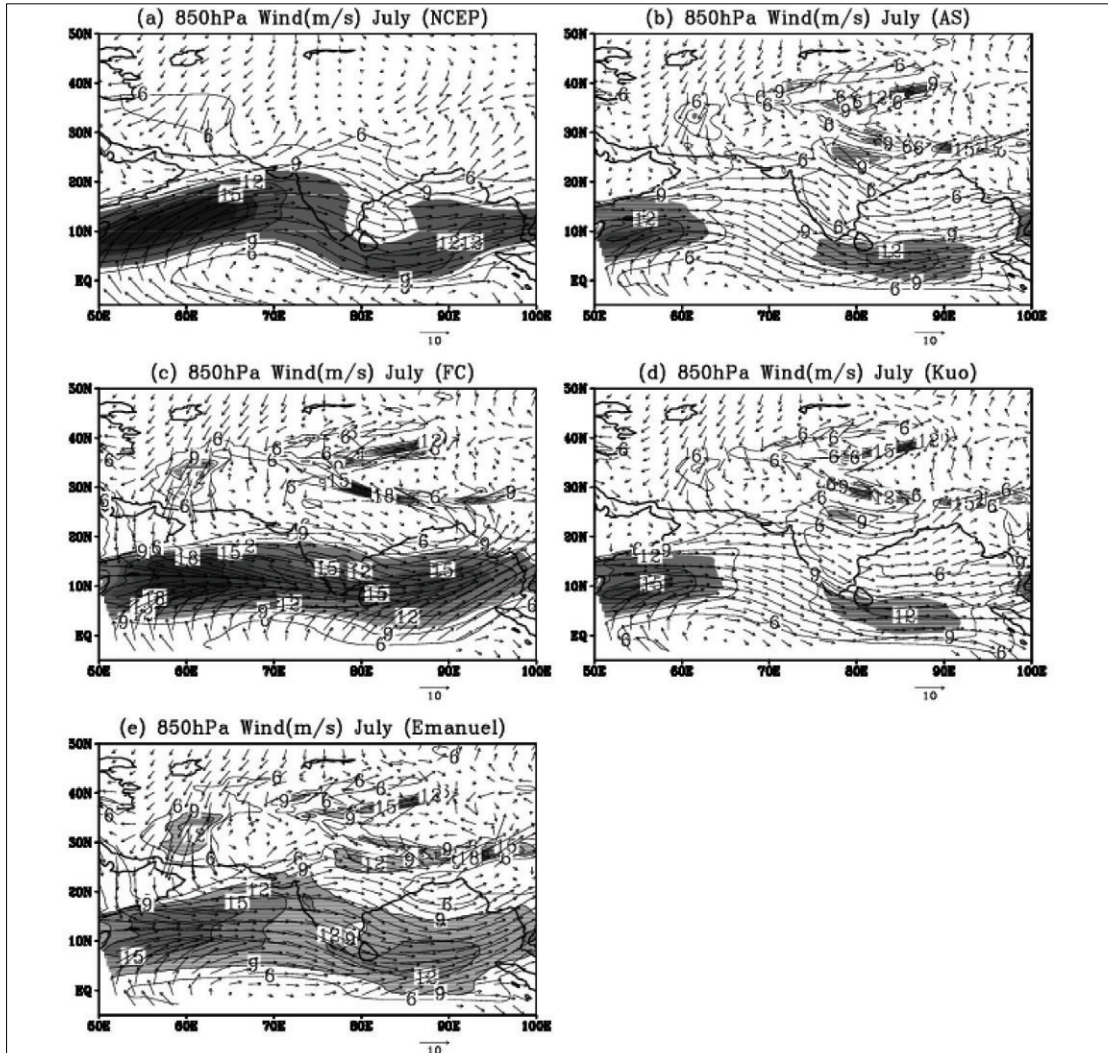
Fig. 1. Wind (m/s) at 850 hPa in July for (a) NCEP (observed), (b) AS closure in Grell, (c) FC closure in Grell, (d) Kuo-type and (e) Emanuel convective schemes respectively. (Wind more than 9m/s are shaded)
