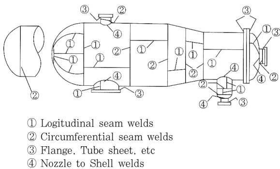
Fig. 1 Classification of weld joint positions in pressure vessel manufacturing
