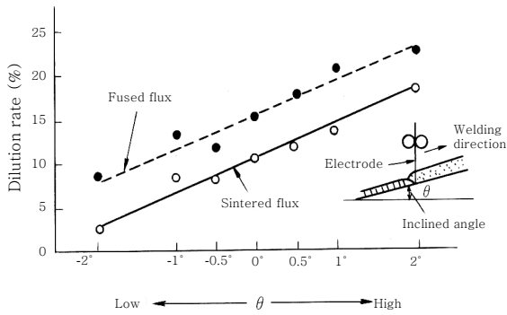
Fig. 7 Variation of dilution rate according to the inclined angle of base metal
