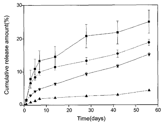
Figure 6. PTX release from various polymer films with 10% PTX: -■- PCL, -▲- PCL/PLGA(50:50), -●- PLGA, and -▼- PLLA.
