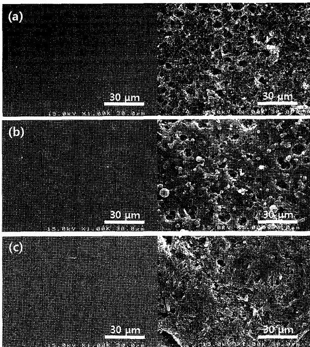
Figure 4. FE-SEM images of different PTX loaded-PLGA films: (a) 5%, (b) 10%, and (c) 15%.
