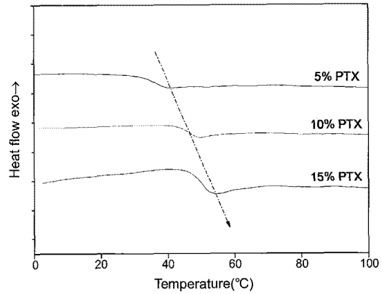
Figure 5. DSC data of PLGA films with various PTX loading.
