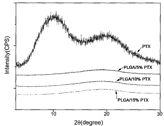
Figure 2. X-ray diffraction data of PLGA films with PTX.
