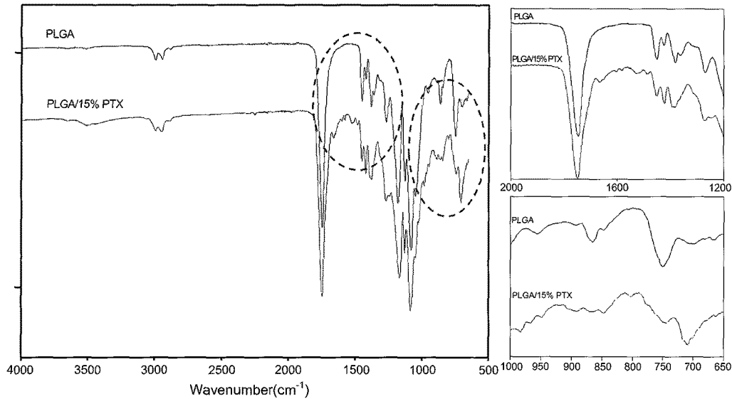
Figure 1. ATR-FTIR spectra of two PLGA films: PLGA and 15% PTX loaded-PLGA film.
