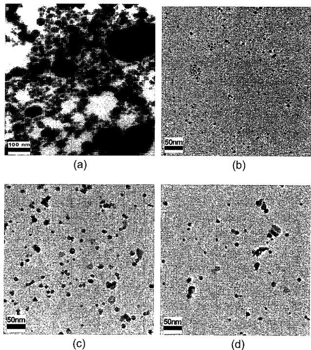
Figure 6. TEM image of (a) Ag/PS(2.0/100) at 110 °C; (b) Ag/PS(1.0/100, microwave); (c) Ag/PS(1.0/100, microwave, 60 °C); (d) Ag/PS(4.0/100, microwave, 60 °C).
