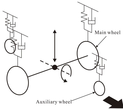
Fig. 1 Schematic of suspension system of intelligent service robot
