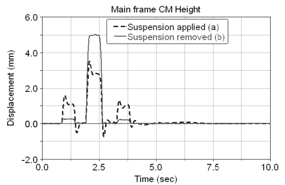
Fig. 5 Main frame height in dynamic analysis of passing over bump
