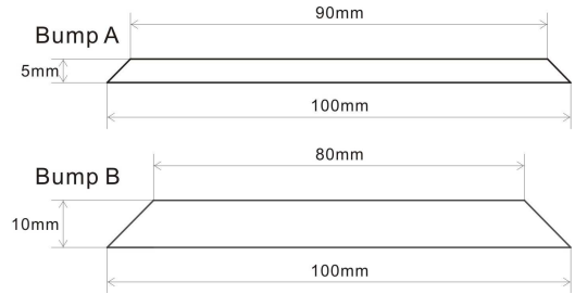
Fig. 3 Bump shapes
