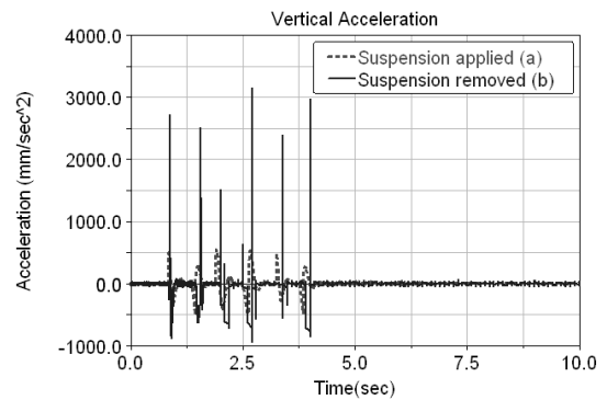
Fig. 4 Vertical acceleration in dynamic analysis of passing over bump
