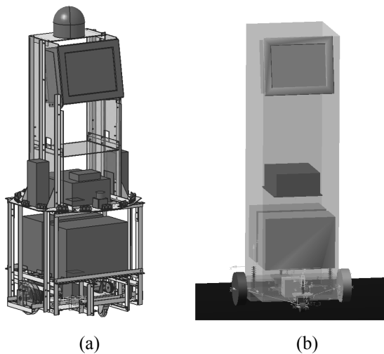
Fig. 2 Internal structure design (a) and dynamic model (b) of intelligent service robot
