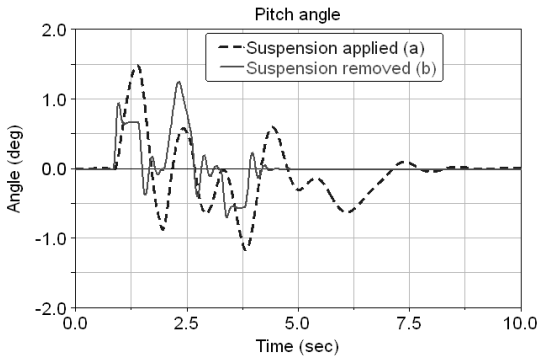
Fig. 6 Pitch angle in dynamic analysis of passing over bump
