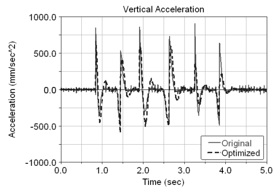
Fig. 9 Optimized vertical acceleration
