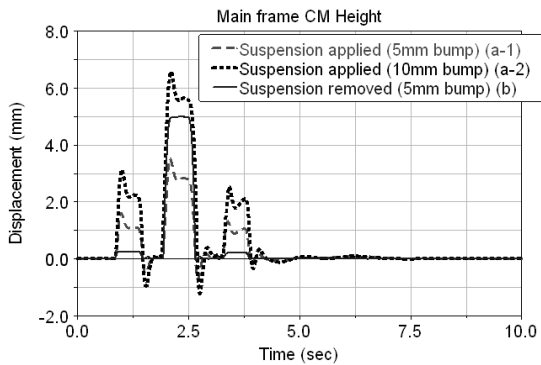
Fig. 7 Main frame height in dynamic analysis of passing over different bumps
