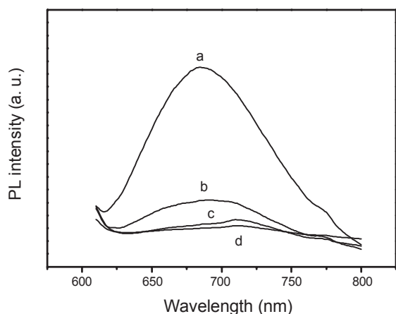
Figure 2. PL emission spectra of various weight ratios of PEC-FTP to PCBM in film: (a) 1:0, (b) 1:1, and (c) 1:3.
