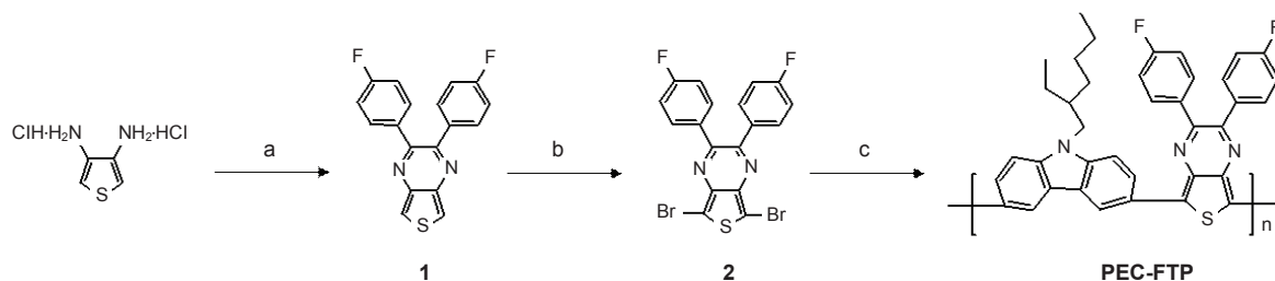
Scheme 1. Synthetic route to PEC-FTP: (a) 4,4'-difluorobenzil, triethylamine, dichloromethane/ethanol (1/1); (b) NBS, DMF; (c) 3,6-bis(4,4,5,5-tetramethyl-1,3,2-dioxaborolane)-9-( N -2-ethylhexyl)carbazole, Pd(PPh 3 ) 4 , K 2 CO 3 , toluene.
