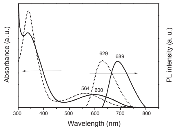
Figure 1. UV-visible absorption and PL emission spectra of PEC-FTP in chloroform (dotted lines) and film (solid lines).
