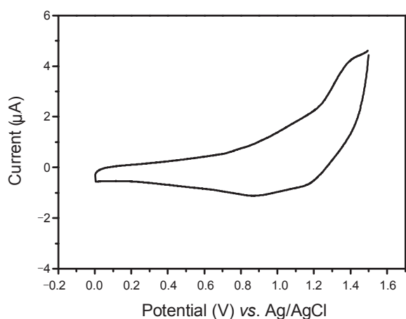
Figure 3. Cyclic voltammogram curve of PEC-FTP in chloroform (0.40 mg/mL) containing 0.10 M Bu 4 NBF 4 .
