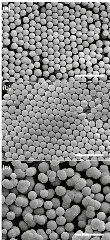
Figure 2. FE-SEM micrographs of silica structures. The volume ratio of water to ethanol: (a) 0.6:1, (b) 0.8:1, and (c) 1:1. The scale bar is 5 \mu\text{m} .
