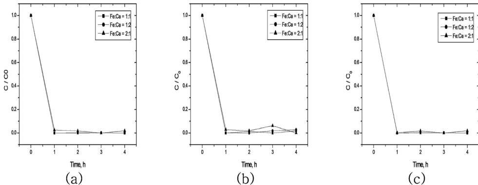
Fig. 4. Reduction of perchlorate ions by Fe-alginate bead at different temperatures. Initial concentration of [ClO 4 - ] was 10 mg/L at pH 7.2. Reaction temperature was 100 (a), 50 (b) and 25 (c) respectively.
