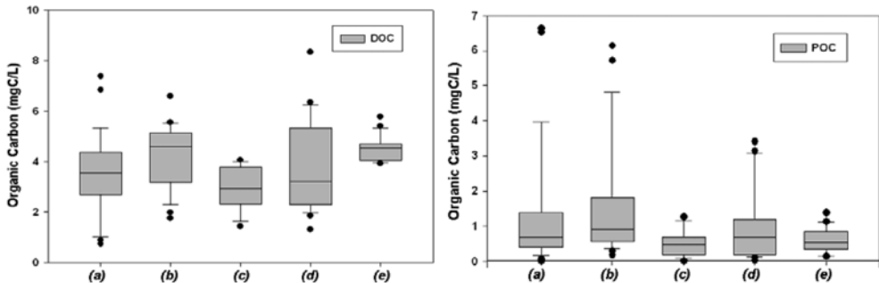
Fig. 2. The comparison of DOC and POC at Youngsan river system: (a) Gwangju-cheon sites, (b) Youngsan river main stream sites, (c) Hwangryong river sites, (d) tributary sites, (e) sewage effluents.
