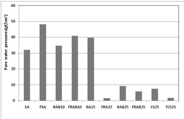
Fig. 7. Reduction of the pore water pressure under condition of sudden draw down
