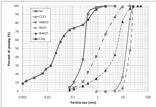
Fig. 1. Grain size accumulation curve
