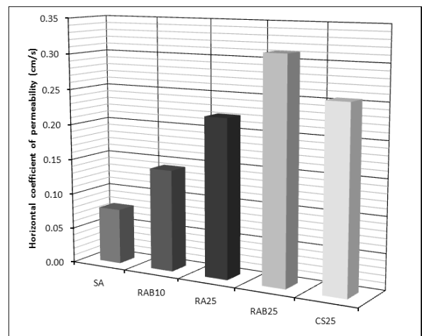
Fig. 4. Horizontal coefficient of permeability for various drains
