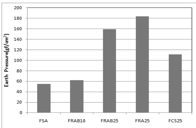
Fig. 12. Reduction of earth pressure under condition of sudden draw down
