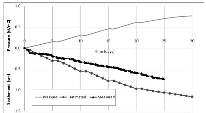
Fig. 9. Variations of the estimated and measured settlement
