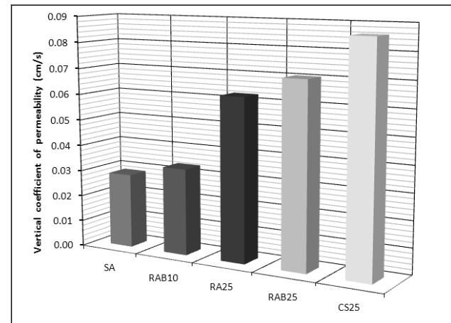
Fig. 5. Vertical coefficient of permeability for various drains
