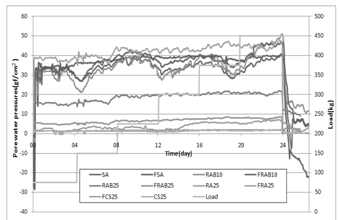
Fig. 6. Variations of pore water pressure with time
