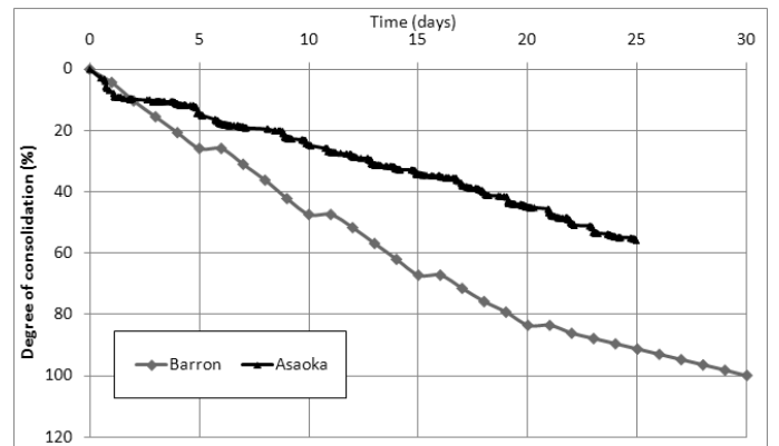
Fig. 10. Variations of the degree of consolidation
