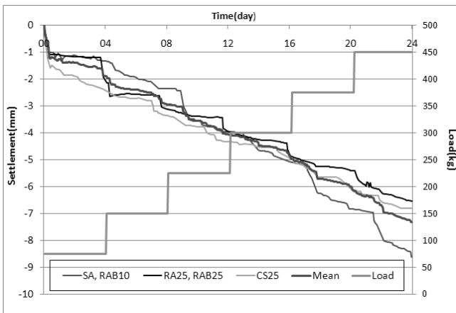
Fig. 8. Variations of settlement with time
