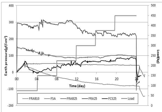
Fig. 11. Variations of earth pressure with time
