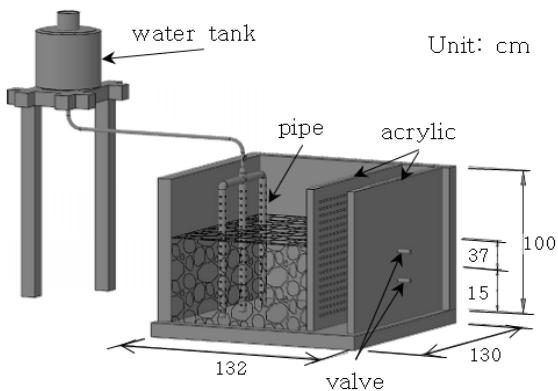
Fig. 3. A cross-section of horizontal permeability test apparatus.
