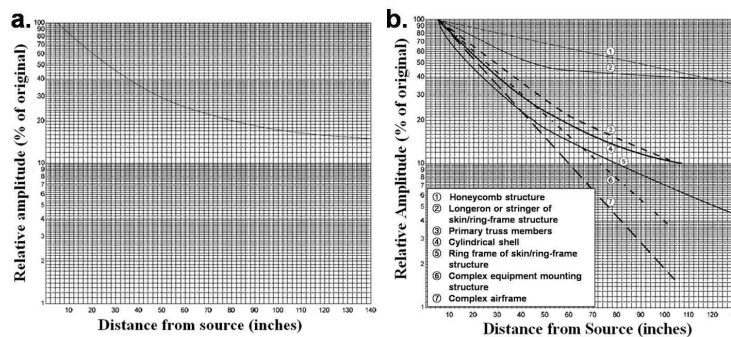
Fig. 5. Shock attenuation due to distance in low and high frequency region [3]
