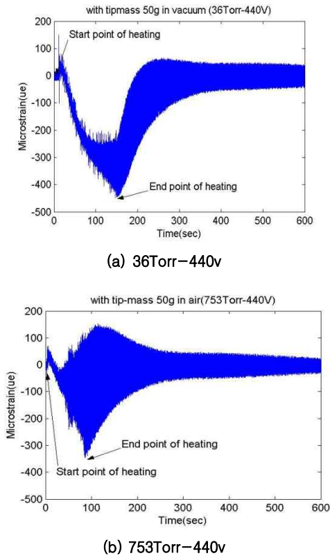
Fig. 7. Variation of thermal strains measured at 2290W-440V lamp power in vacuum and atmosphere
