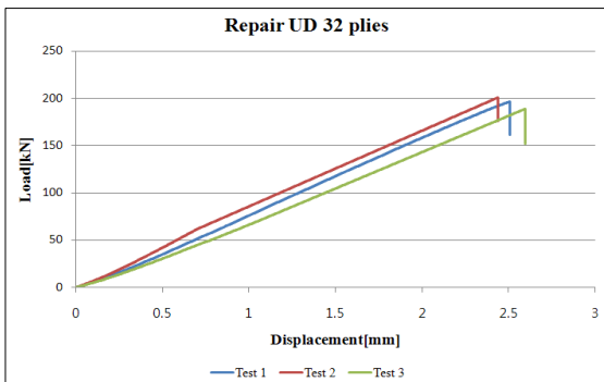
Fig. 12 Load-displacement curves of compressive test after repair.
