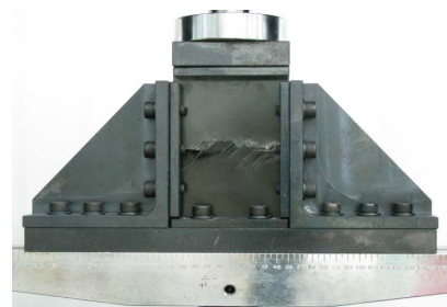
(b) after compressive test
