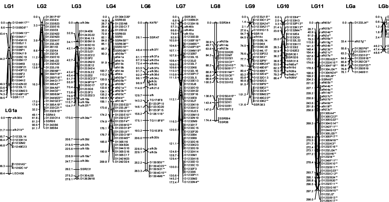
Fig. 1. Genetic linkage map of 362 loci in 188 F 9 recombinant inbred lines derived from a cross between S. lycopersicum H7996 and S. pimpinellifolium WVa700. Map distances are shown in centimorgans (cM) on the left side of the linkage groups and were calculated using the Kosambi mapping function. Loci marked with * and ** deviate significantly from 1:1 ratio at P < 0.01 and P < 0.001, respectively.
