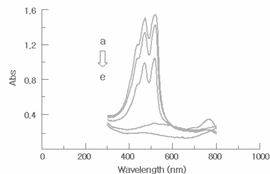
Fig. 7. Absorption spectra of PProDOP-Oct (top) and PProDOP-Dod (bottom) in 50 mM \text{LiClO}_4 at the potential of (a) -0.6, (b) -0.4, (c) -0.2, (d) +0.4, and (e) +0.4 V.
