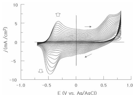
Fig. 4. Cyclic voltammograms during electrochemical synthesis of PProDOP-Oct on Au in acetonitrile/H 2 O cosolvent (1/1) of 50 mM LiClO 4 . \nu = 50 mVs -1 .
