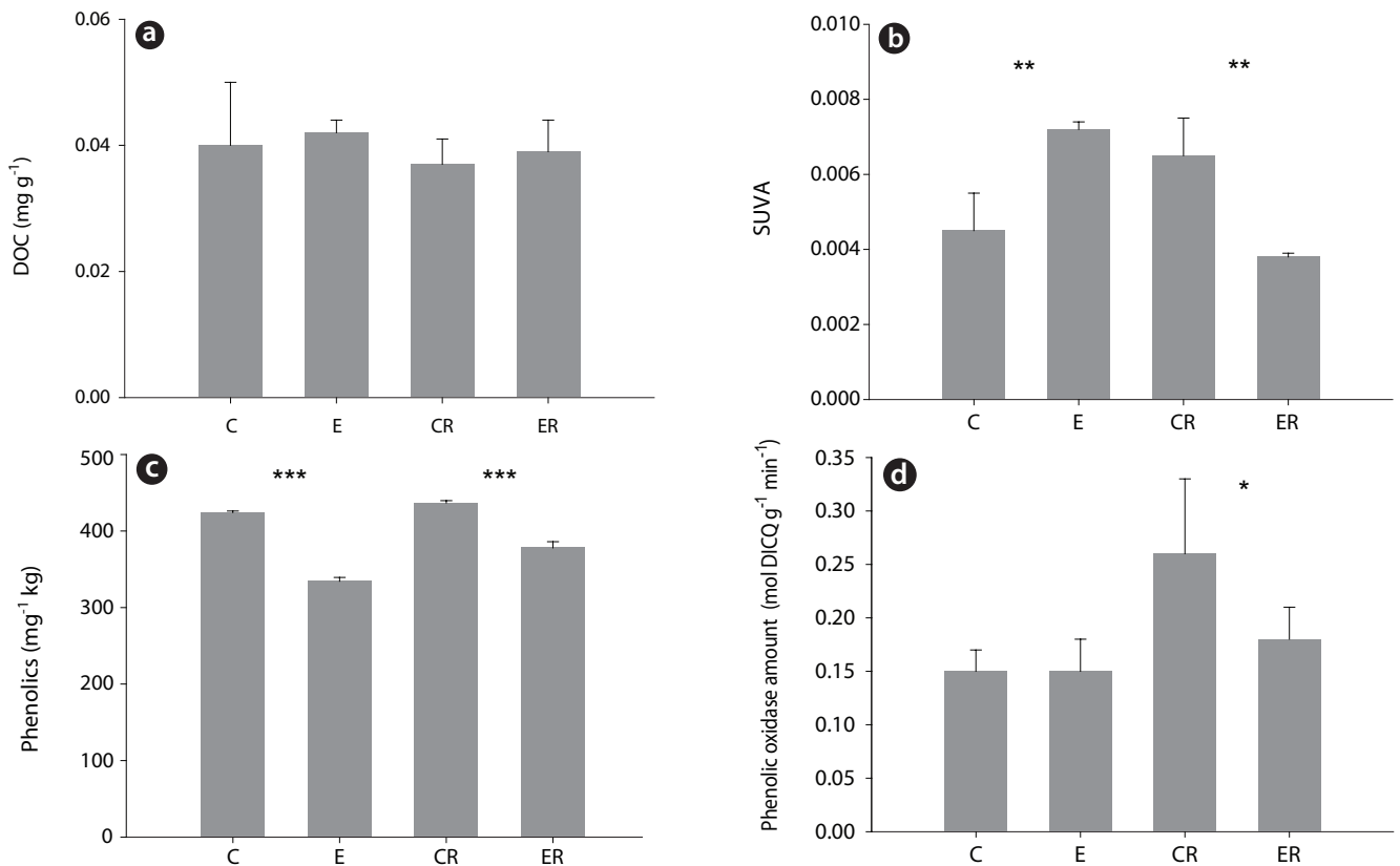
Fig. 2. (a) Dissolved organic carbon concentration, (b) specific UV absorbance (SUVA 254 ), (c) phenolic compounds, and (d) phenolic oxidase activity after 12 months. C, 380 ppmv, bulk soil; CR, 380 ppmv, rhizosphere soil; E, 760 ppmv, bulk soil; ER, 760 ppmv, rhizosphere soil.
