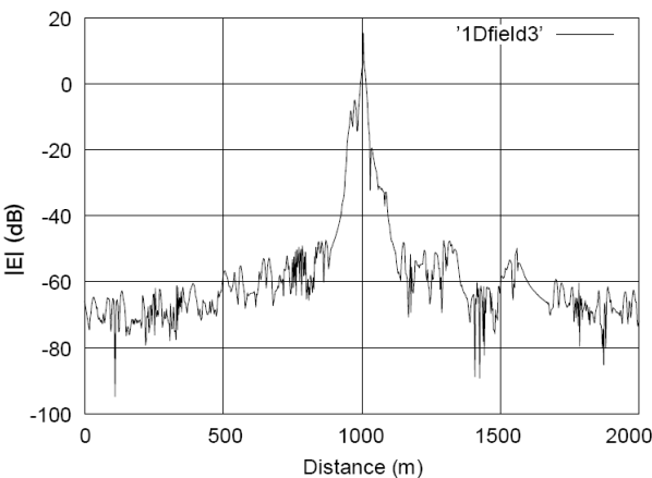
그림 6 전계강도(In case of third order ray) Fig. 6 Field computed by third order ray.
