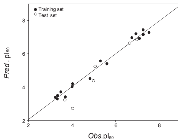
Figure 2. Relationships between observed activities ( Obs.pI_{50} ) against the cucumber and predicted activities ( Pred.pI_{50} ) by the CoMSIA model I. (For the training set: Pred.pI_{50} = 0.985Obs.pI_{50} + 0.08 , n = 16 , S = 0.218 , F = 858.893 , r^2 = 0.984 and q^2 = 0.981 ).
