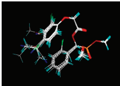
Figure 1. Alignment of the potential energy minimized O,O -dialkyl-1-phenoxyacetoxy-1-methyl-phosphonate substrate structures according to a least-squares atom based fit.
