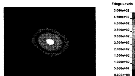
Fig. 2 Von Mises Stress Results for Aluminum Plate ( t=0.005\text{ms} , V=1000\text{m/s} ).
