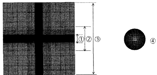
Fig. 1 Mesh and Dimension of Model.
