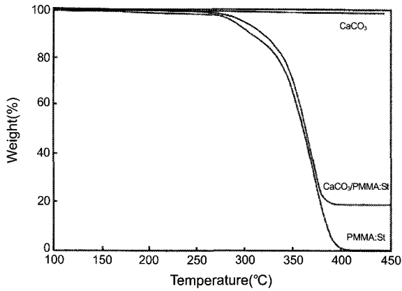
Figure 6. TGA curves of \text{CaCO}_3 , \text{CaCO}_3/\text{PMMA}:\text{PSt} core-shell and PMMA homopolymer.
