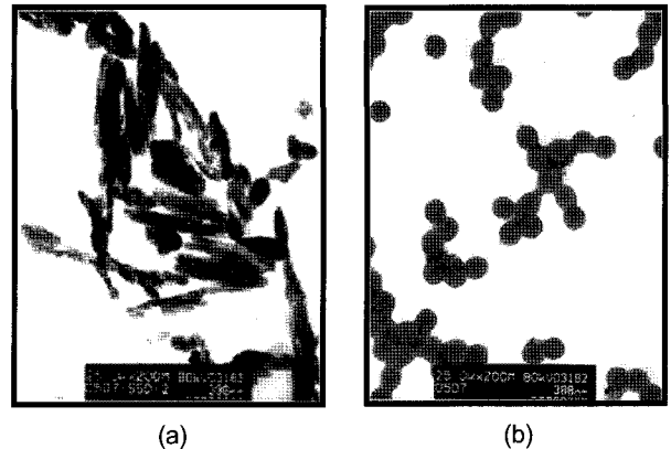
Figure 8. TEM micrograph of (a) \text{CaCO}_3 ; (b) \text{CaCO}_3/\text{PMMA}:\text{PSt} core-shell particle.
