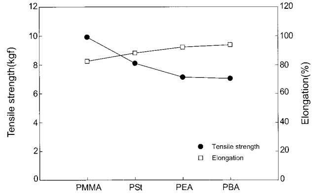
Figure 10. Tensile strength and elongation of core-shell particle.
