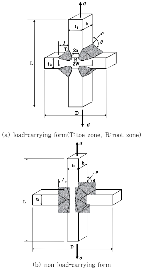
Fig. 2 Configuration of cruciform fillet joints
