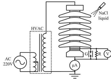
Fig. 2. Configuration of the experimental apparatus.
