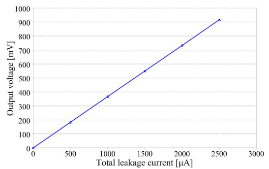
Fig. 5. Output voltage as a function of total leakage current.
