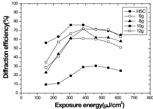
Fig. 4. Diffraction efficiency of HAAC.
