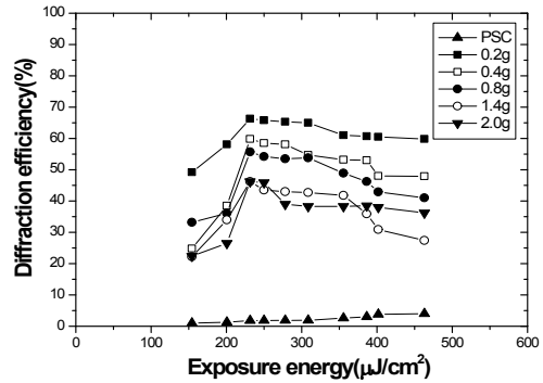
Fig. 3. Diffraction efficiency of PAAC.
