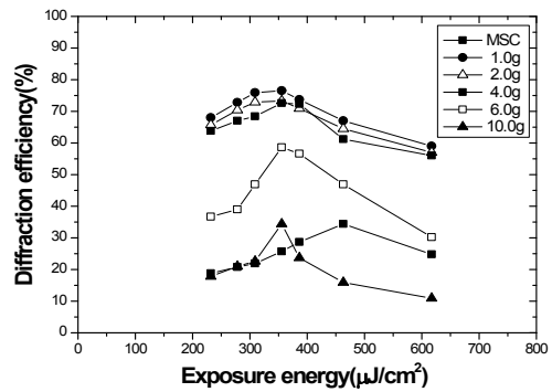
Fig. 2. Diffraction efficiency of MAA.
