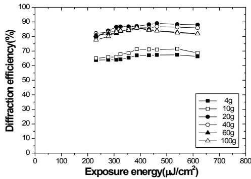
Fig. 1. Diffraction efficiency of AAC.
