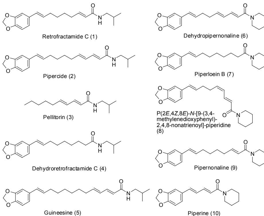
Figure 1. The chemical structures of ten alkamides isolated from P. longum and P. nigrum .
