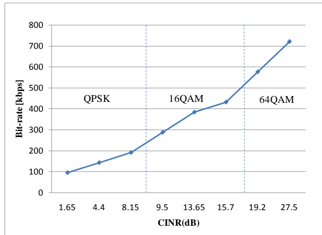
Fig. 2. Bit-rate level as CINR with AMC mode
