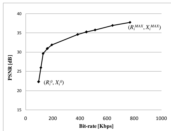
Fig. 3. R-D curve of “Habour” sequence
