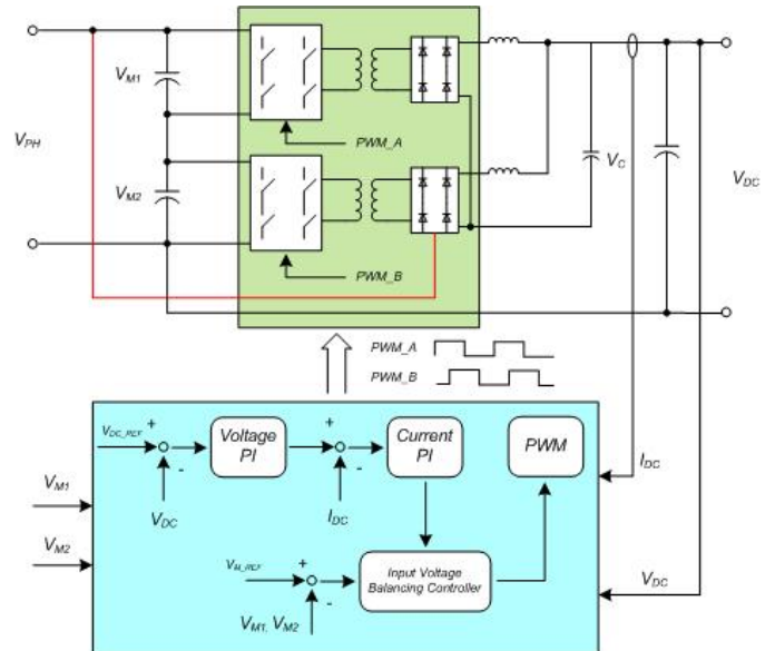
Fig. 5. Block diagram of the proposed ISOP converter controller.
