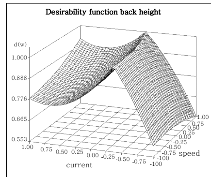
(b) Desirability function for back bead height (variables : welding current and speed)
