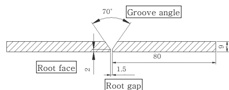
Fig. 2 Configuration of butt welding specimen (250×80×9mm)
