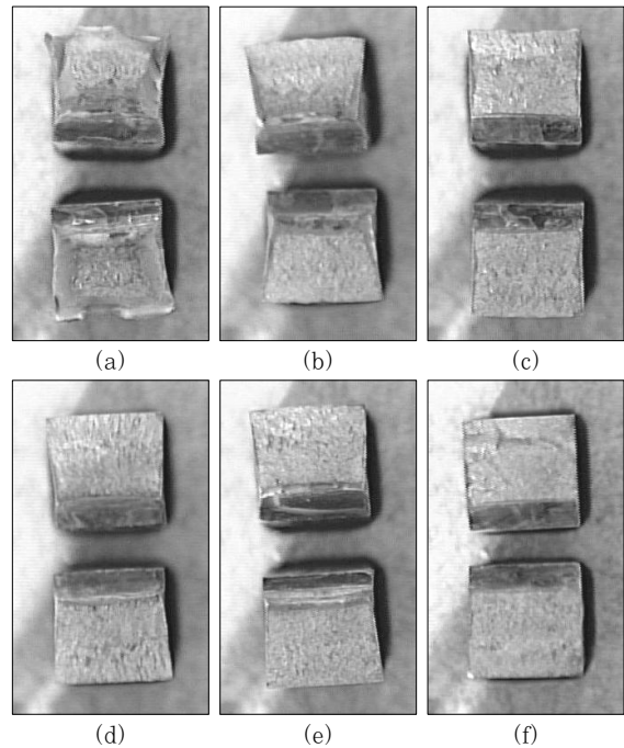
Fig. 9 Macrographs showing irradiated standard CVN impact specimens tested at different temperatures(x2). (a) 0, (b) -20, (c) -30, (d) -50, (e) -60 and (f) -80°C
