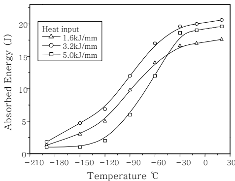
Fig. 3 Absorbed energy vs. temperatures of weld subsize CVN specimens with different heat inputs
