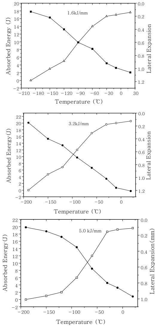
Fig. 6 Absorbed energy and lateral expansion of weld subsized CVN specimens as a function of heat inputs (a) 1.6, (b) 3.2 and (c) 5.0 kJ/mm
