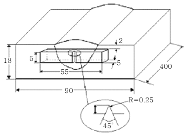
Fig. 1 Schematic diagram of subsized Charpy V notch impact test specimen in the weld joint geometry(unit: mm)
