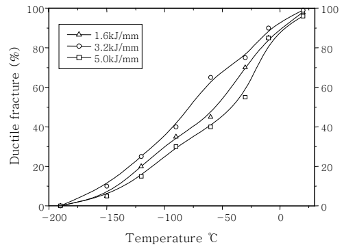
Fig. 5 Proportion of ductile fracture of subsize CVN specimens
