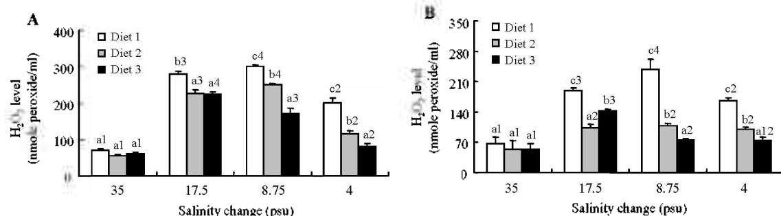
Figure 4. Plasma H_2O_2 concentrations in olive flounder fed a diet containing quercetin (Diet 2, 0.25%; Diet 3, 0.5%) or no quercetin (Diet 1, 0%) for 30 (A) or 60 days (B) and then exposed to seawater (35 psu) and osmotic stress (17.5, 8.75, and 4 psu). Values with alphabets indicate significant differences between Diet 1, 2 and 3 within the same time after exposure. The numbers indicates significant differences from the control (within the same diet) ( p < 0.05 ). All values are means \pm SD ( n = 5 ).
