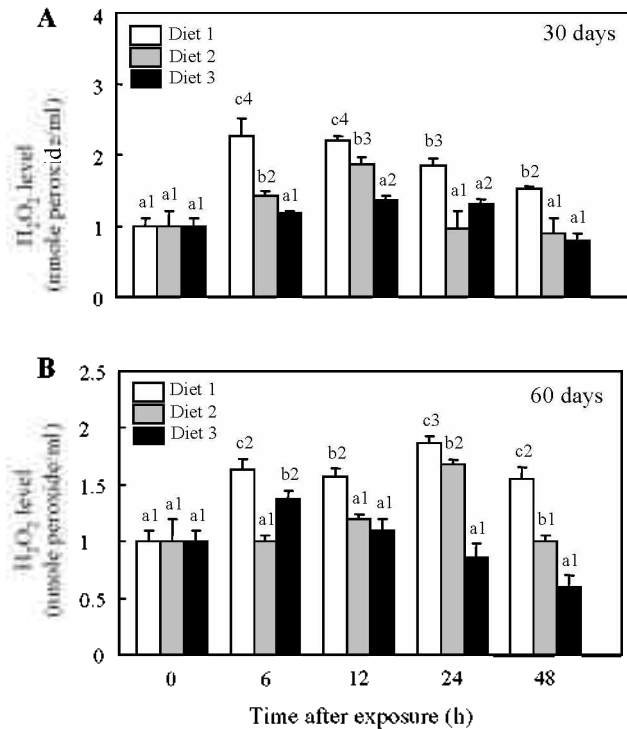
Figure 5. H_2O_2 concentrations in plasma of olive flounder fed for 30 or 60 days diets containing quercetin 0.25 or 0.5%, after 6, 12, 24, and 48 h exposure to Cd. Values with alphabets indicate significant differences between Diet 1, 2 and 3 within the same time after exposure. The numbers indicate a significant difference from the control (within the same diet) ( p < 0.05 ). All values are means \pm SD ( n = 5 ).
