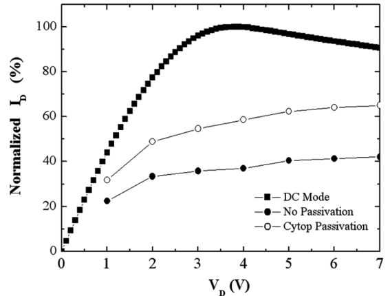
Fig. 3. Gate lag measurements on unpassivated and Cytop™ passivated HEMTs (1.2×200 μm 2 gate). V G was switched from -4.5 to 0 V.
