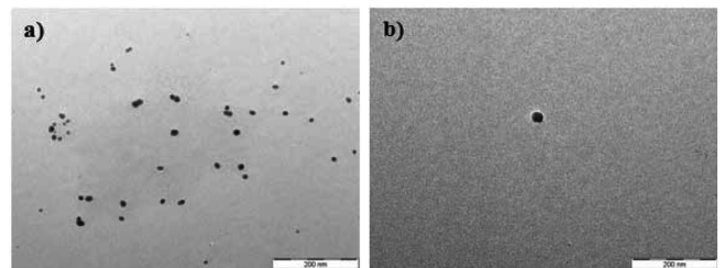
Fig. 5. TEM analysis of WPU/silica nanocomposites prepared with different amounts of TEOS in Table 2. a)T0 and b)T8.
