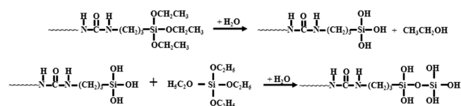
Scheme 2. The scheme to prepare waterborne polyurethane/silica nanocomposites.
