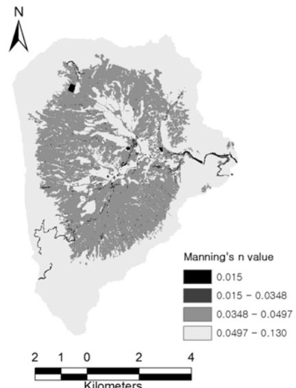
Fig. 11. Manning's n grid.
