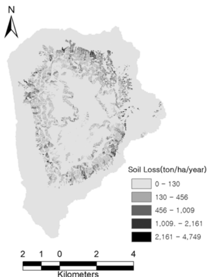
Fig. 10. Soil Loss Estimated using the SATEEC
