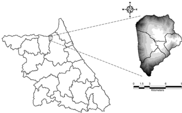
Fig. 1. Location of Haeam-myeon watershed.
