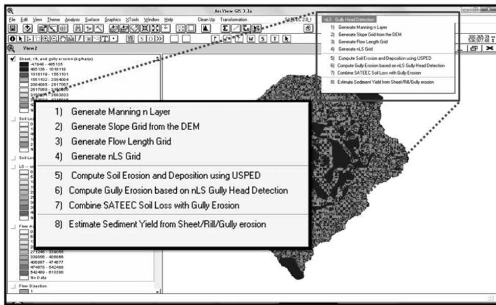
Fig. 9. Interface of integrated system using SATEEC, nLS, and USPED.
