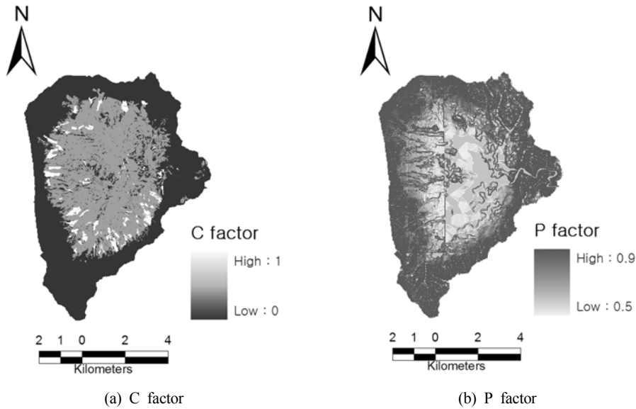
Fig. 5. USLE C and P factors in SATEEC system.
