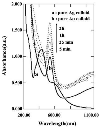
Fig. 1. UV-visible spectra recorded as a function of reaction time of Au/Ag bimetallic nanocolloids formed with 1 mM HAuCl 4 and then 1 mM AgNO 3 by 5% Magnolia kobus leaf broth at 60 °C. Curve a and b represent UV-visible spectra of pure silver and gold nanocolloids, respectively.
