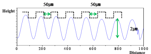
FIG. 7. Surface profile on the gap-electrode pattern
