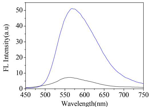
FIG. 5. Fluorescence intensity of the unpatterned (black) and patterned (blue) area. Excited at 415 nm (1000x).
