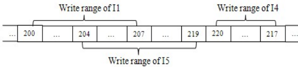
(Fig. 2) The reallocation of expanded frequent page set. Write range of I1 is expanded to sector 100~119. For the reallocation, sector 100~119 is moved to 200~219 and sector 35~42 is moved to sector 220~217
