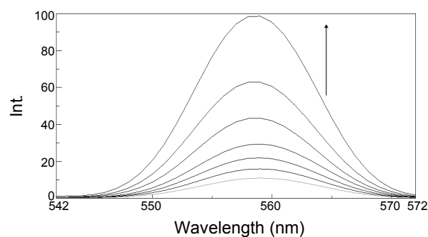
Fig. 7. Emission spectra of PhCH 2 Co(DH) 2 SCNCo(DH) 2 U complex in aqueous buffer at pH 7.2 in the presence of CT-DNA. Arrow shows the intensity change upon increasing DNA concentrations
