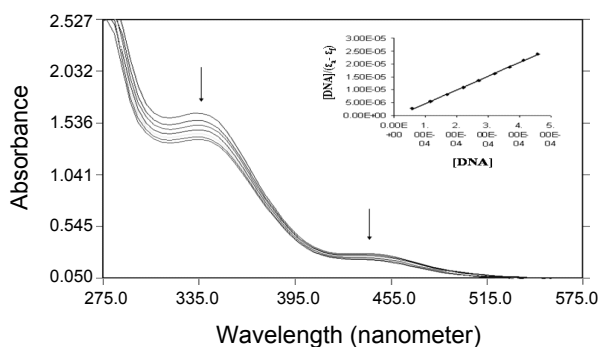
Fig. 6. Absorption spectra of PhCH 2 Co(DH) 2 SCNCo(DH) 2 U (top) in the absence of CT DNA, the absorbance changing upon increasing CT DNA concentrations. The arrow shows the intensity change upon increasing DNA concentration
