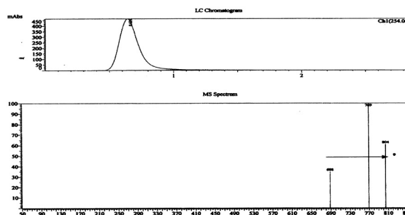
Fig. 5. LC/MS spectra of [PhCH 2 Co(DH) 2 SCNCo(DH) 2 TU] complex.
