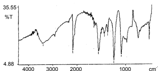
Fig. 3. IR spectra of [PhCH 2 Co(DH) 2 SCNCo(DH) 2 AC].
