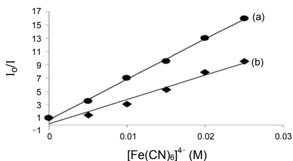
Fig. 8. Emission quenching curves of complex in absence of DNA (a) presence of DNA (b).
