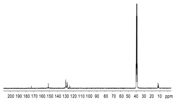
Fig. 2. 13 C [ 1 H] NMR spectra of PhCH 2 Co(DH) 2 SCNCo(DH) 2 SC complex in DMSO- d 6 .
