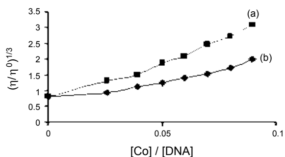
Fig. 9. Effect of increasing amounts of ethidium bromide (a) and complex (b) PhCH 2 Co(DH) 2 SCNCo(DH) 2 U on the relative viscosity of CT DNA at 25 ± 0.1 °C.
