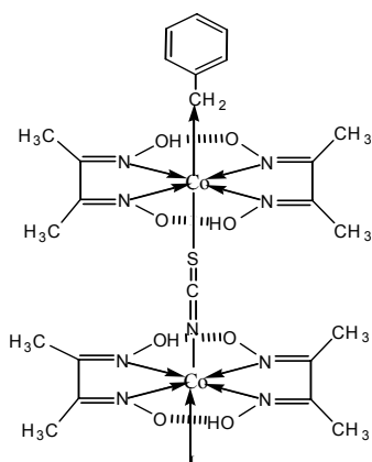
Structure 1. Thiocyanato bridged (benzyl ligand) dicobaloximes
