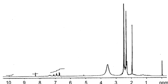
Fig. 4. 1 H NMR spectra of [PhCH 2 Co(DH) 2 SCNCo(DH) 2 U] complex in DMSO- d 6 .
