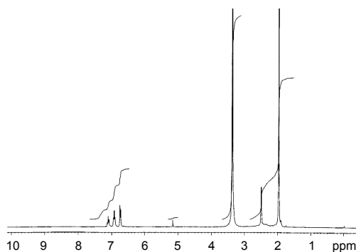
Fig. 1. 1 H NMR spectra of benzyl(aquo) cobaloxime in DMSO- d 6 .
