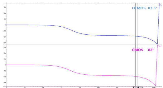
Fig. 10. Phase margin(deg) compared with the DT-CMOS and CMOS error amplifier
