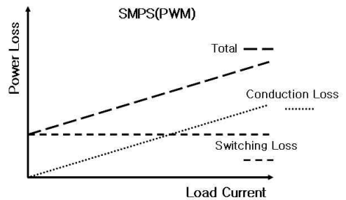
Fig. 1. Analysis of SMPS efficiency loss
