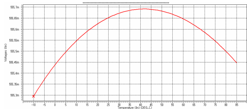
Fig. 14. Reference voltage change with temperature
