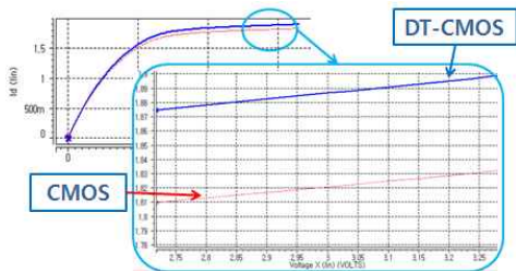
Fig. 7. I-V characteristics of DT-CMOS and CMOS
