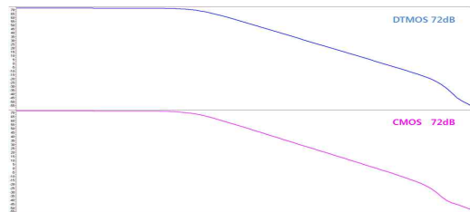
Fig. 9. DC gain compared with the DT-CMOS and CMOS error amplifier
