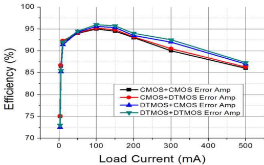
Fig. 11. The efficiency of Buck converter with load current variation
