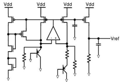
Fig. 13. Low voltage reference generator circuit
