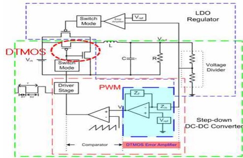
Fig. 12. Whole block diagram of DC-DC converter
