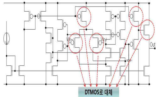
Fig. 8. Proposed DT-CMOS error amplifier
