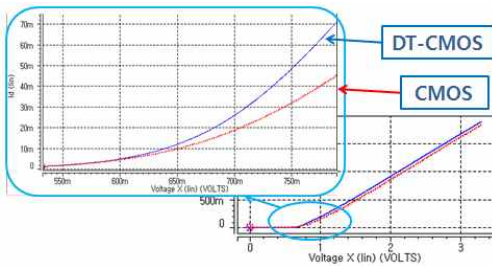
Fig. 6. Threshold voltage comparison of DT-CMOS and CMOS
