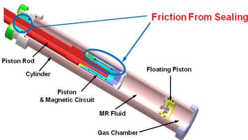
Fig. 2 Configuration of the conventional MR damper
