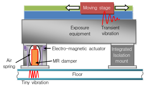
Fig. 1 Configuration of the integrated isolation mount
