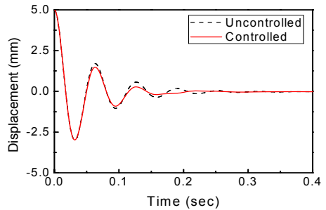
(a) Displacement vs. time
