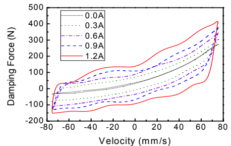
(c) Damping force vs. velocity
