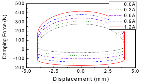
(b) Damping force vs. displacement
