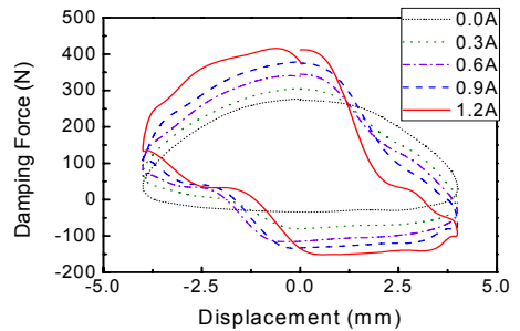
(b) Damping force vs. displacement
