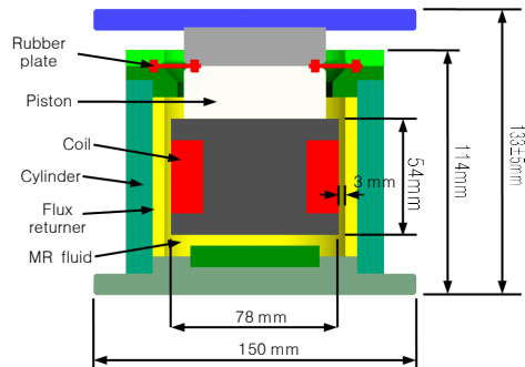
Fig. 4 Design of the proposed MR damper
