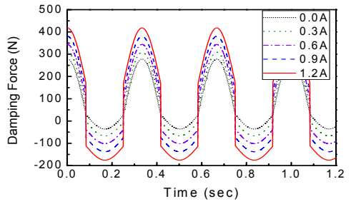
(a) Damping force vs. time
