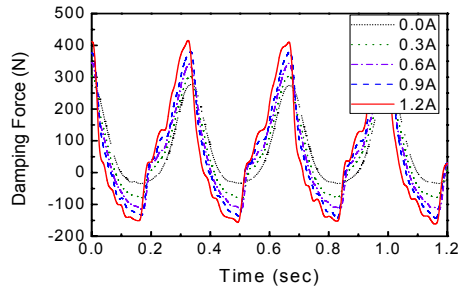
(a) Damping force vs. time
