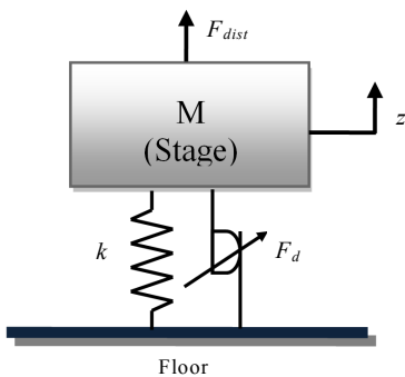
Fig. 9 Mechanical model of the stage with MR damper
