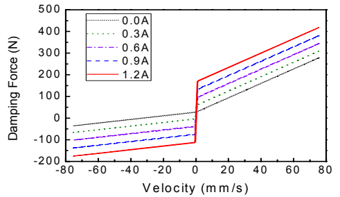
(c) Damping force vs. velocity
