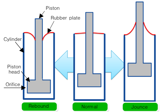
Fig. 3 Configuration of the proposed MR damper
