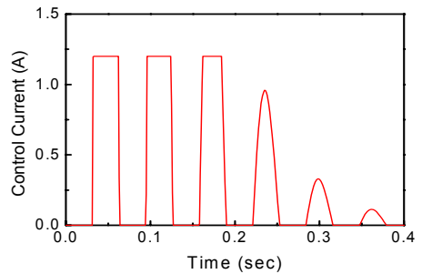
(b) Control current
