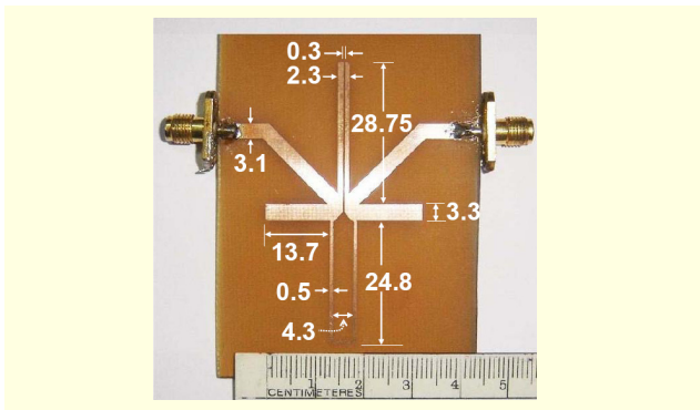
Fig. 4. Photograph of the fabricated LPF.
