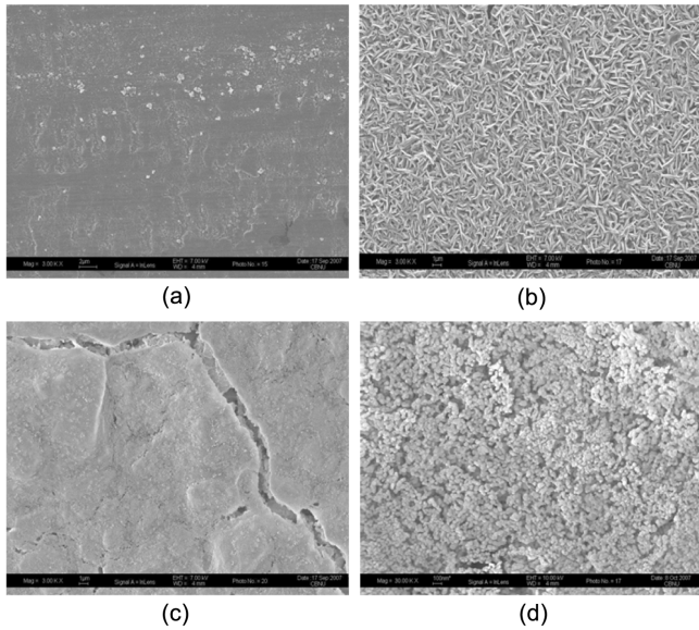
Fig. 5. SEM images of metal monolith with surface treatment (a) root, (b) after pre-oxidation at 1050, (c) after Al 2 O 3 coating, (d) after Ni(15wt%)/Ce 0.80 Zr 0.20 O 2 catalyst coating.
