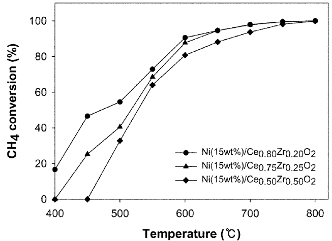
Fig. 6. Temperature dependence of CH 4 conversion over various Ce/Zr ratio (reaction conditions: GHSV=30,000 h -1 , S/C=2, O/C=0.5).
