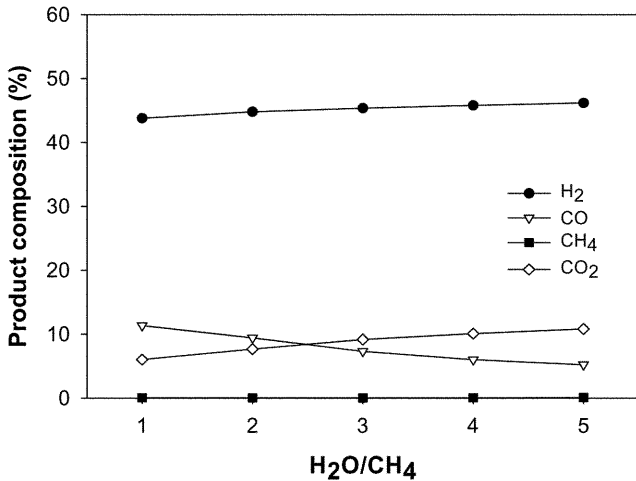
Fig. 10. H 2 O/CH 4 ratio dependence of product composition over Ni (15 wt%)/Ce 0.80 Zr 0.20 O 2 catalyst for the ATR (reaction conditions : Temperature=800 °C, GHSV=30,000 h -1 , O/C=0.5).
