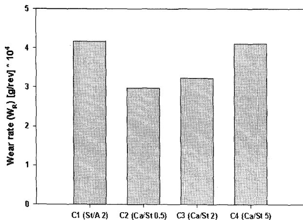
Figure 11. Wear rate with different amount of calcium stearate.
