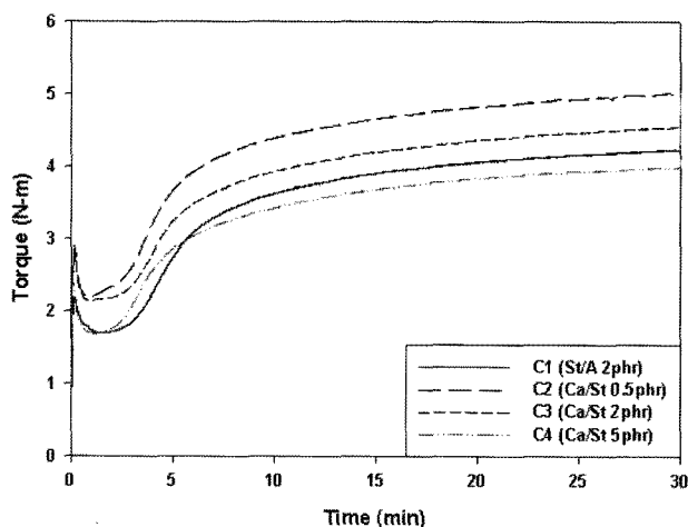
Figure 8. Rheometer curves with different amount of calcium stearate.
