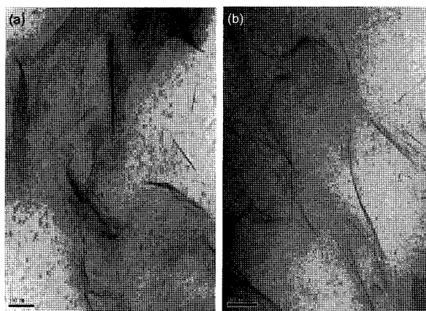
Figure 2. TEM images of (a) SBR/Na-MMT and (b) SBR/DDA-MMT nanocomposites.
