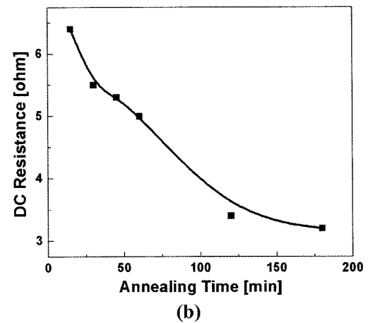
Fig. 1. Relationship between dc resistance and annealing parameters.
