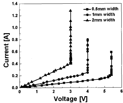
Fig. 5. Maximum current density measurement of P-FCB.
