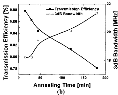
Fig. 3. Frequency characteristics of P-FCB according to (a) Annealing temperature with 20 minutes annealing time (b) Annealing time with 200°C annealing temperature.
