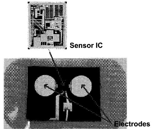
Fig. 10. ECG sensor node using P-FCB [4].
