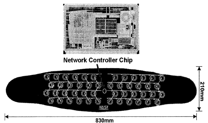
Fig. 11. Inductor channel array implemented on the chest band [4].
