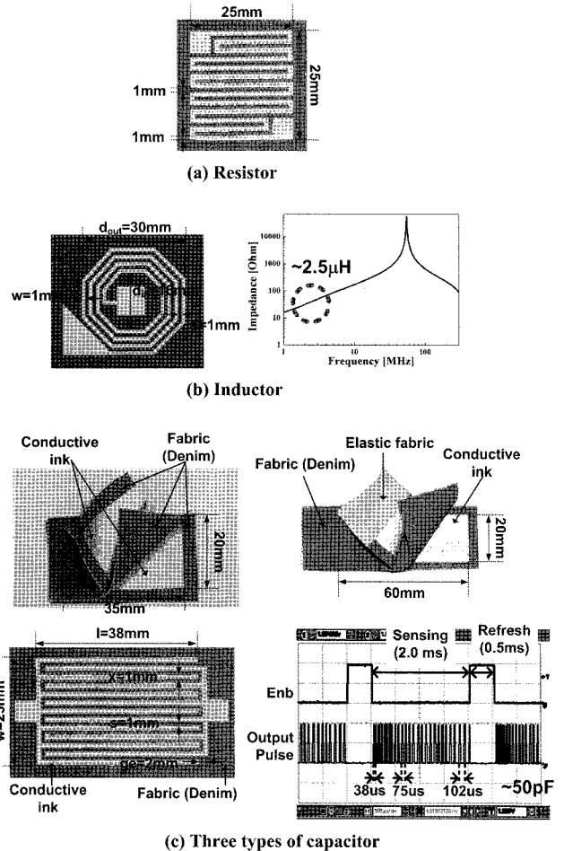
Fig. 9. Passive devices using P-FCB.
