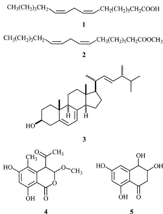
Fig. 1. Structures of compounds 1-5.
