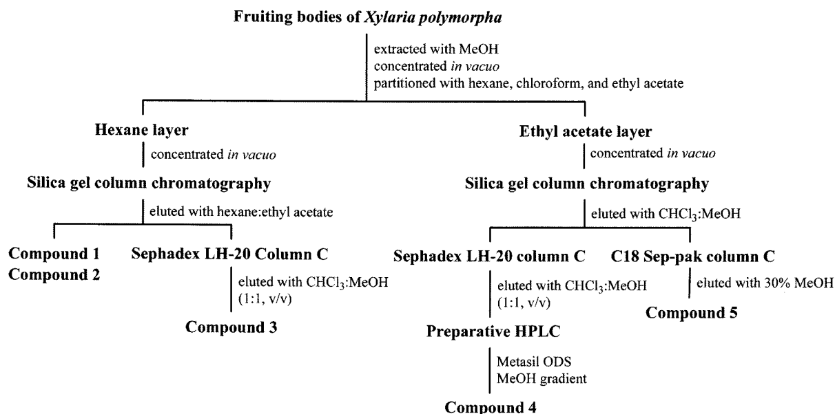
Fig. 2. Isolation procedures of compounds 1~5.
