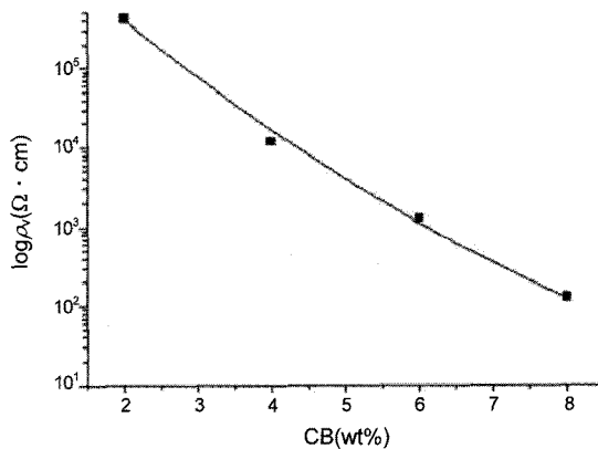
Figure 3. Resistivity of CB composites.
