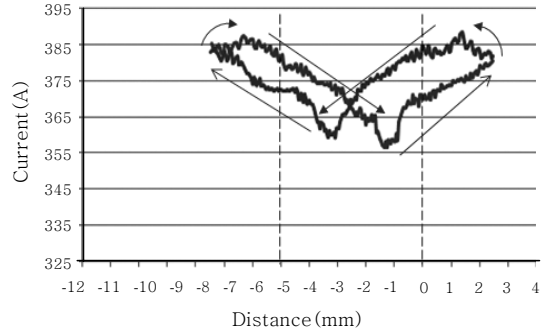
Fig. 11 Peak current waveform for 45° groove angle and 5mm root gap
