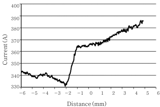
Fig. 7 Peak currents for the bevel angle of 30°
