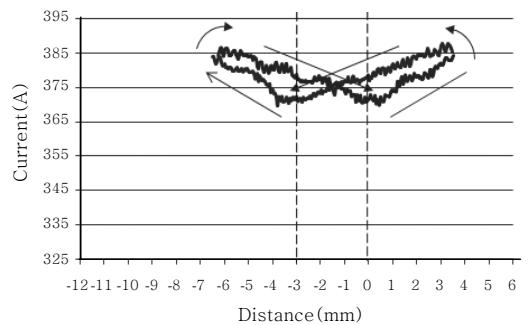
Fig. 13 Peak current waveform for 60° groove angle and 3mm root gap
