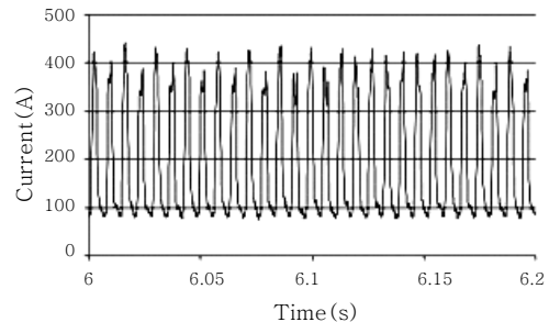
(a) Measured pulse signal
