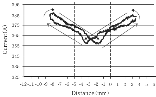
Fig. 14 Peak current waveform for 60° groove angle and 5mm root gap
