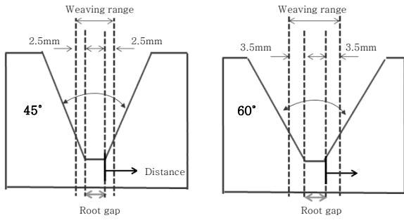
Fig. 9 Configuration of V groove joint
