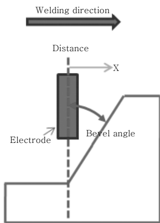
Fig. 3 Configuration of single-sided asymmetric workpiece
