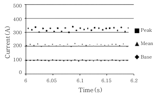
(b) Separated pulse signal
